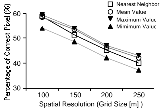
Figure 3. Accuracy of Slope Aspect according to Spatial Resolution
