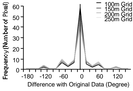
Figure 2. Accuracy of Slope Aspect according to Spatial Resolution
