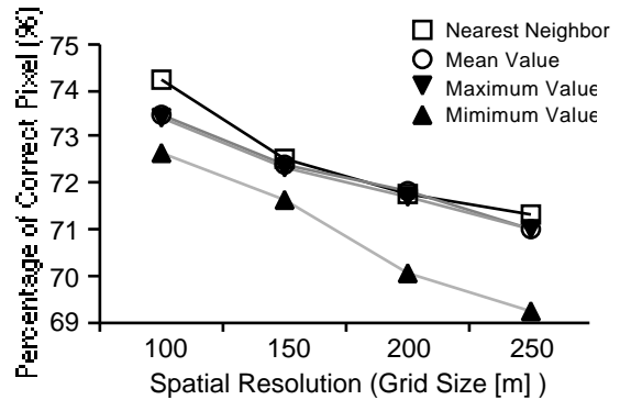
Figure 10. Accuracy of Drainage Pattern according to Spatial Resolution
