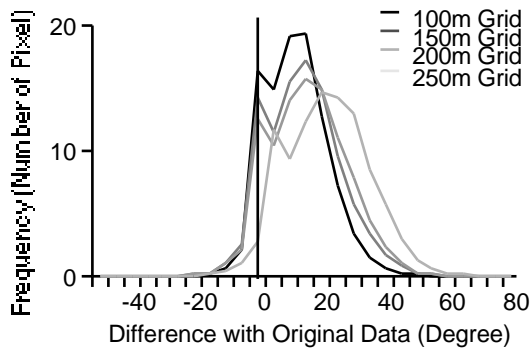
Figure 4. Accuracy of Slope Inclination according to Spatial Resolution
