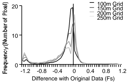
Figure 7. Accuracy of Safety Factor according to Spatial Resolution
