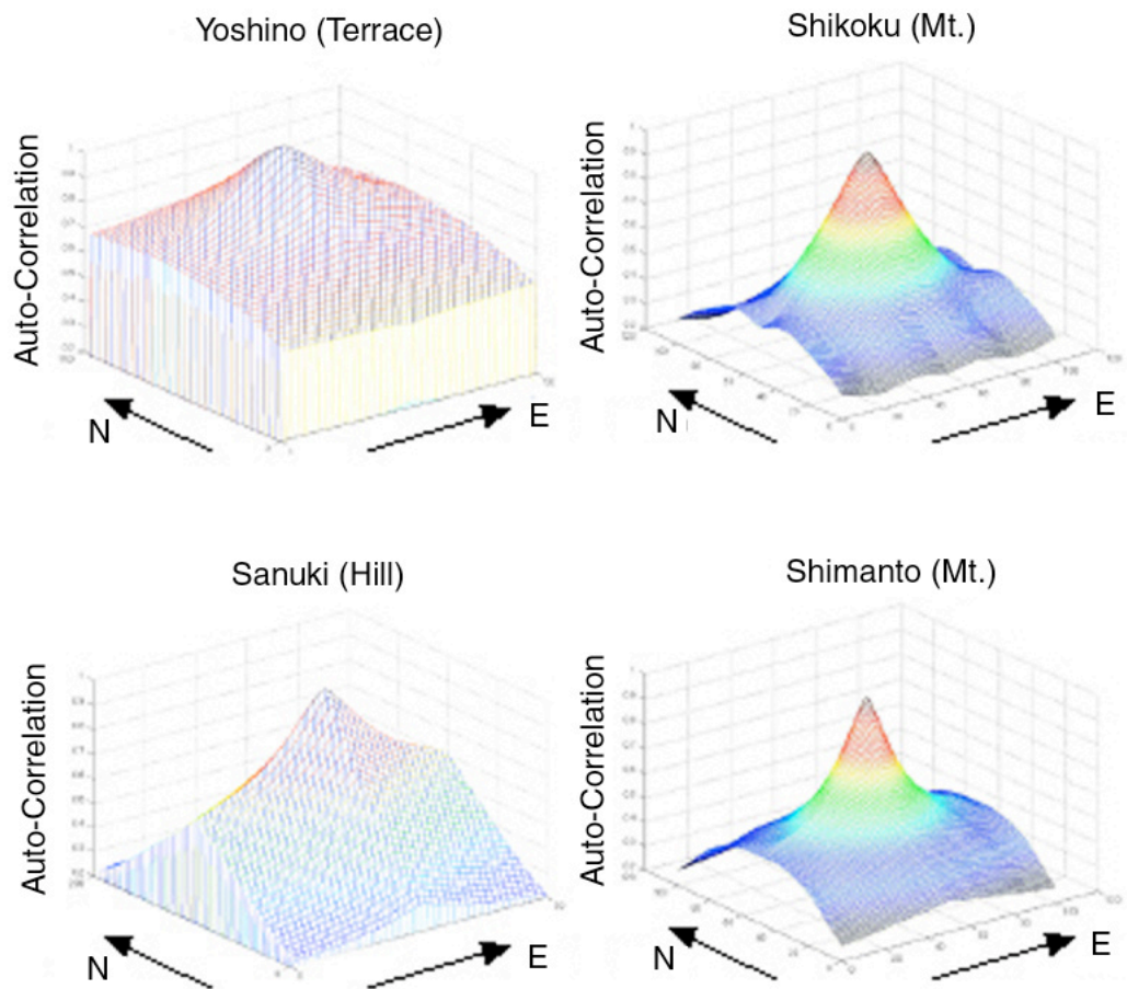
Figure 3. Auto-Correlation of Each DEM
