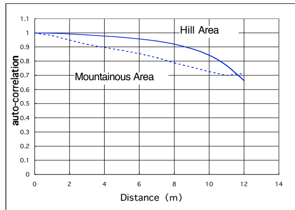
Techniques and Application, Quality Standards, Figure 6. Auto-correlation Function
